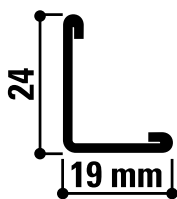
L19x24 C
